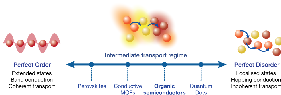
Figure 1: While transport mechanisms are well understood in the extremes, coherent band conduction through extended states and incoherent hopping through localised states, they remain poorly understood in the intermediate regime where many organic semiconductors lie. Figure adapted with permission from (Balzer et al., 2021).
